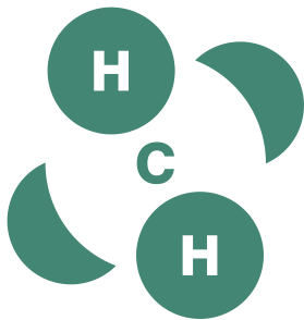
Molecules
